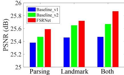
Figure 6: Ablation study on effects of estimated priors.
